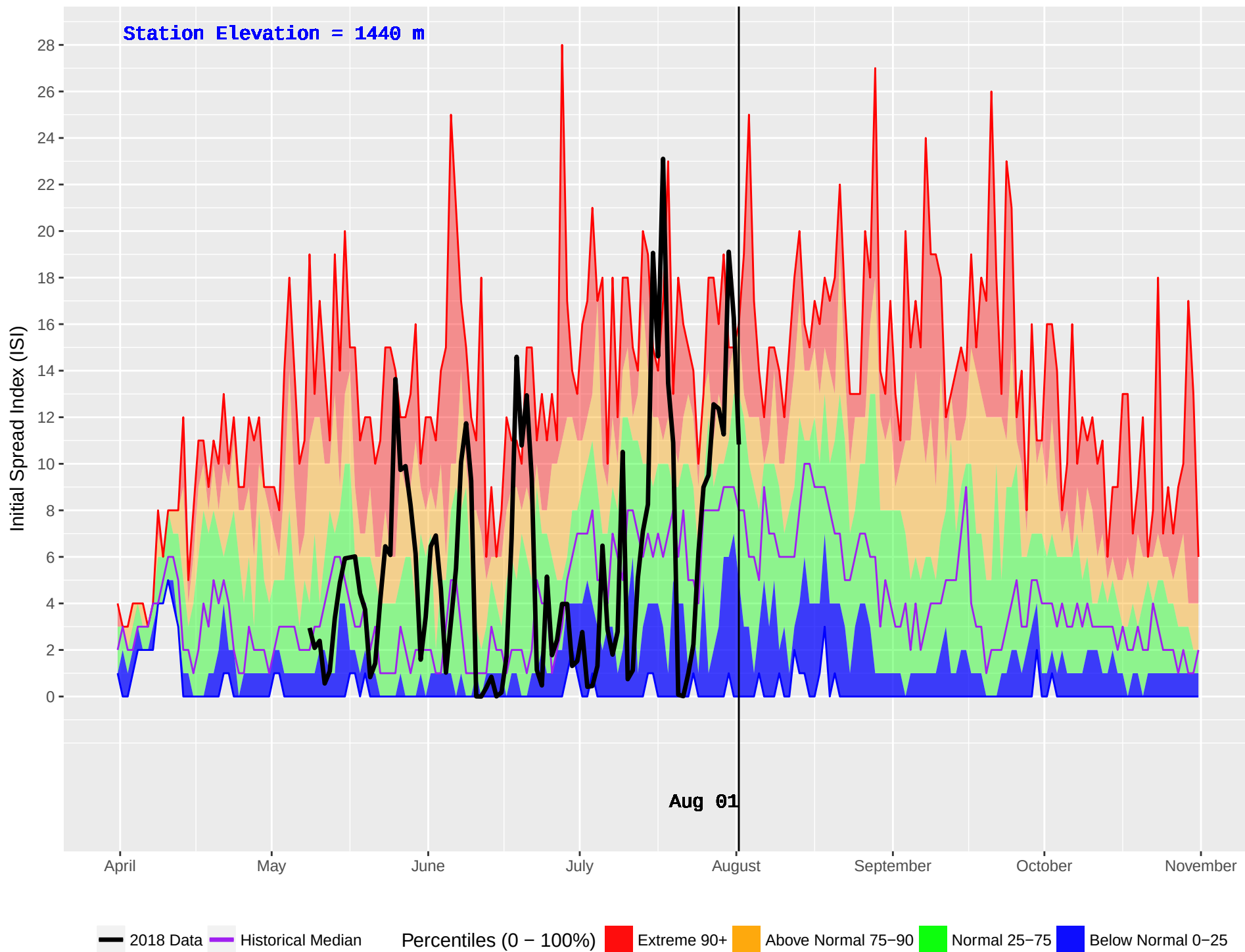
PASKA LAKE (326) : Historical (1999–2016) and Current (2018) Daily Initial Spread Index (ISI)
