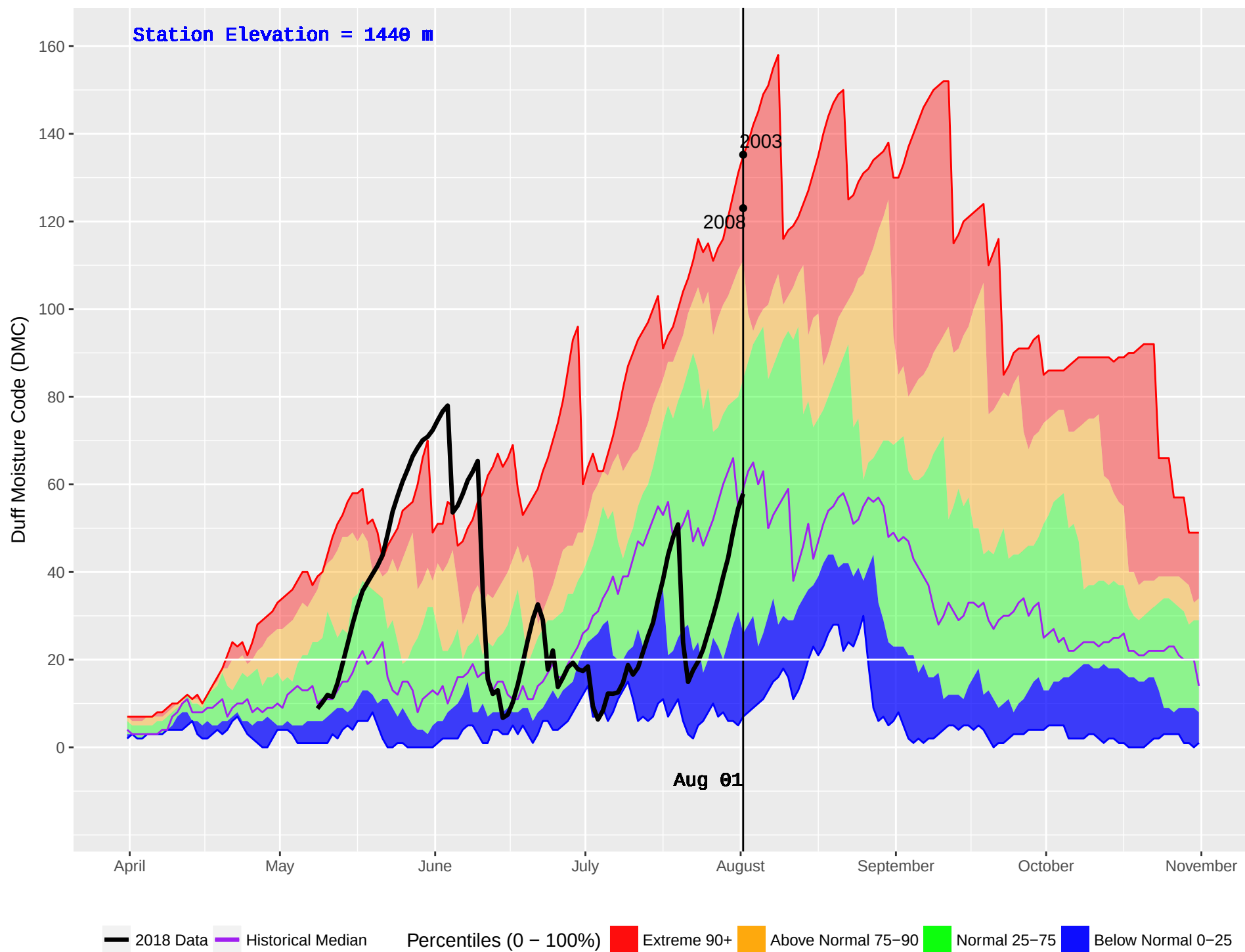
PASKA LAKE (326) : Historical (1999–2016) and Current (2018) Daily Duff Moisture Code (DMC)
