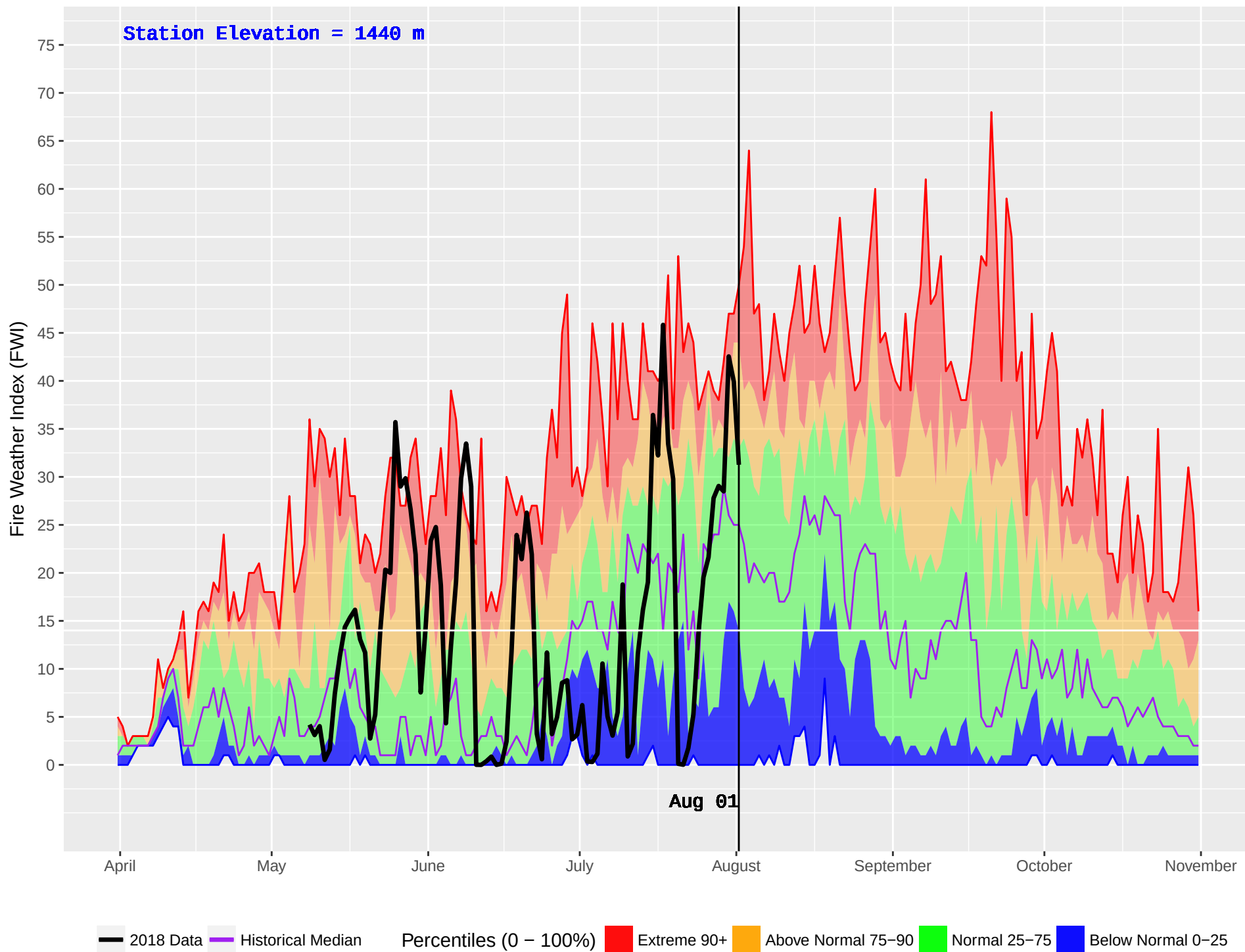
PASKA LAKE (326) : Historical (1999–2016) and Current (2018) Daily Fire Weather Index (FWI)
