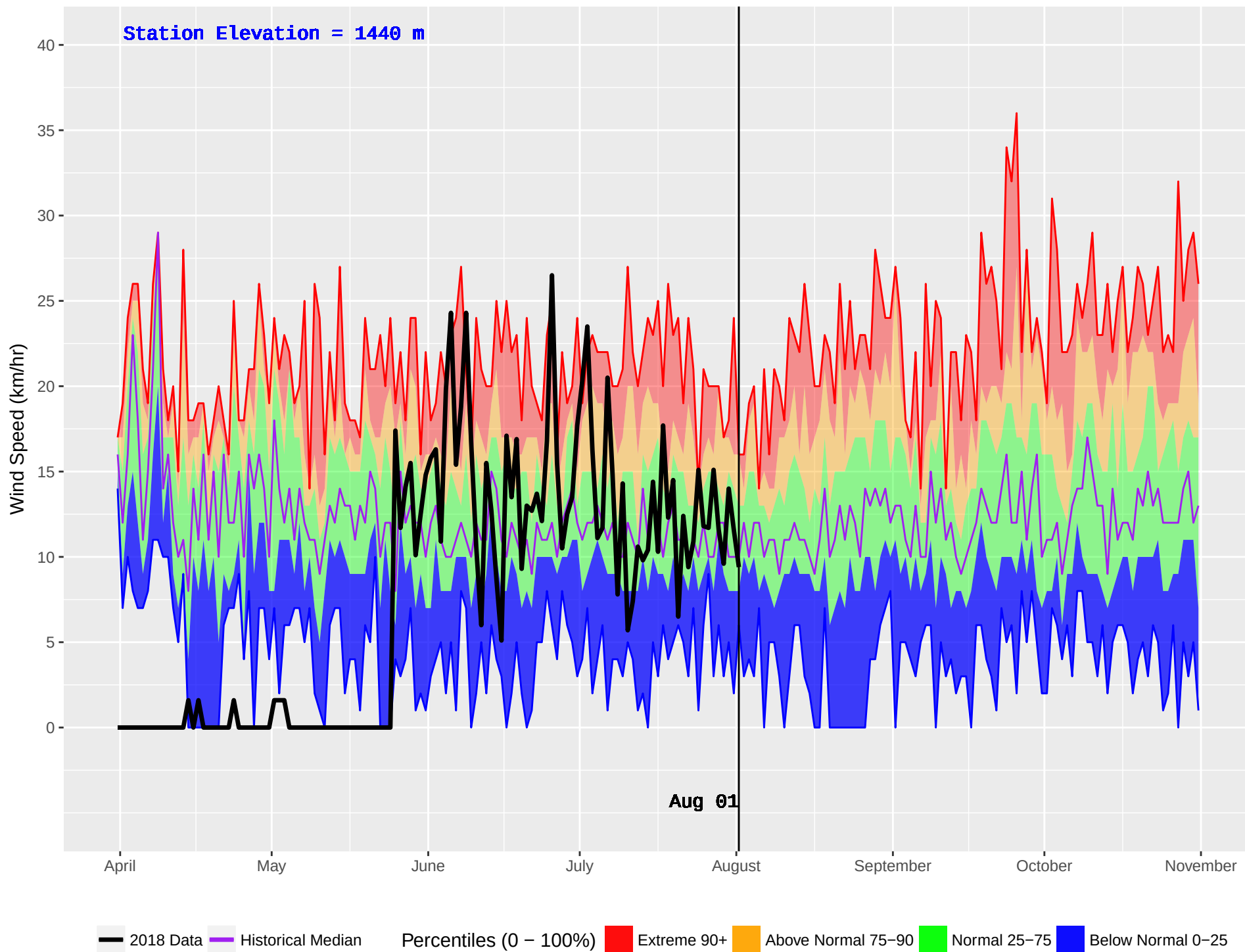
PASKA LAKE (326) : Historical (1999–2016) and Current (2018) Daily Wind Speed
