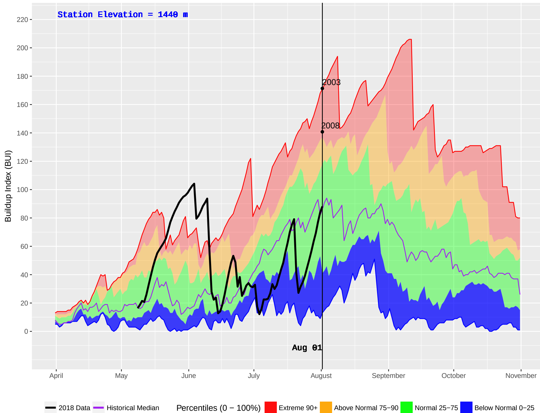
PASKA LAKE (326) : Historical (1999–2016) and Current (2018) Daily Buildup Index (BUI)
