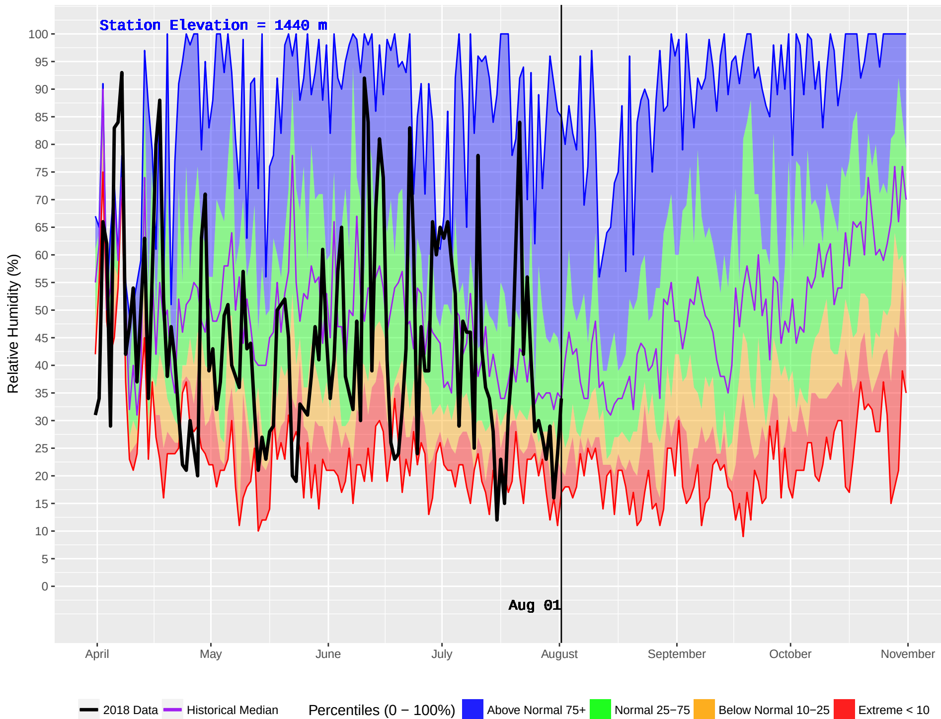
PASKA LAKE (326) : Historical (1999–2016) and Current (2018) Daily Relative Humidity
