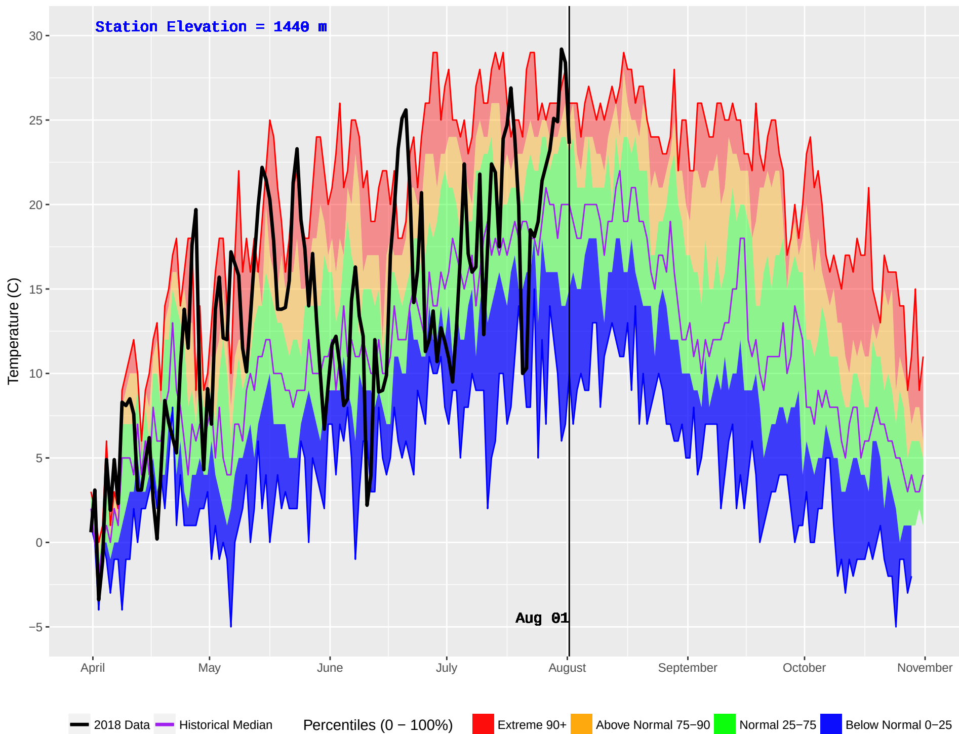
PASKA LAKE (326) : Historical (1999–2016) and Current (2018) Daily Temperature
