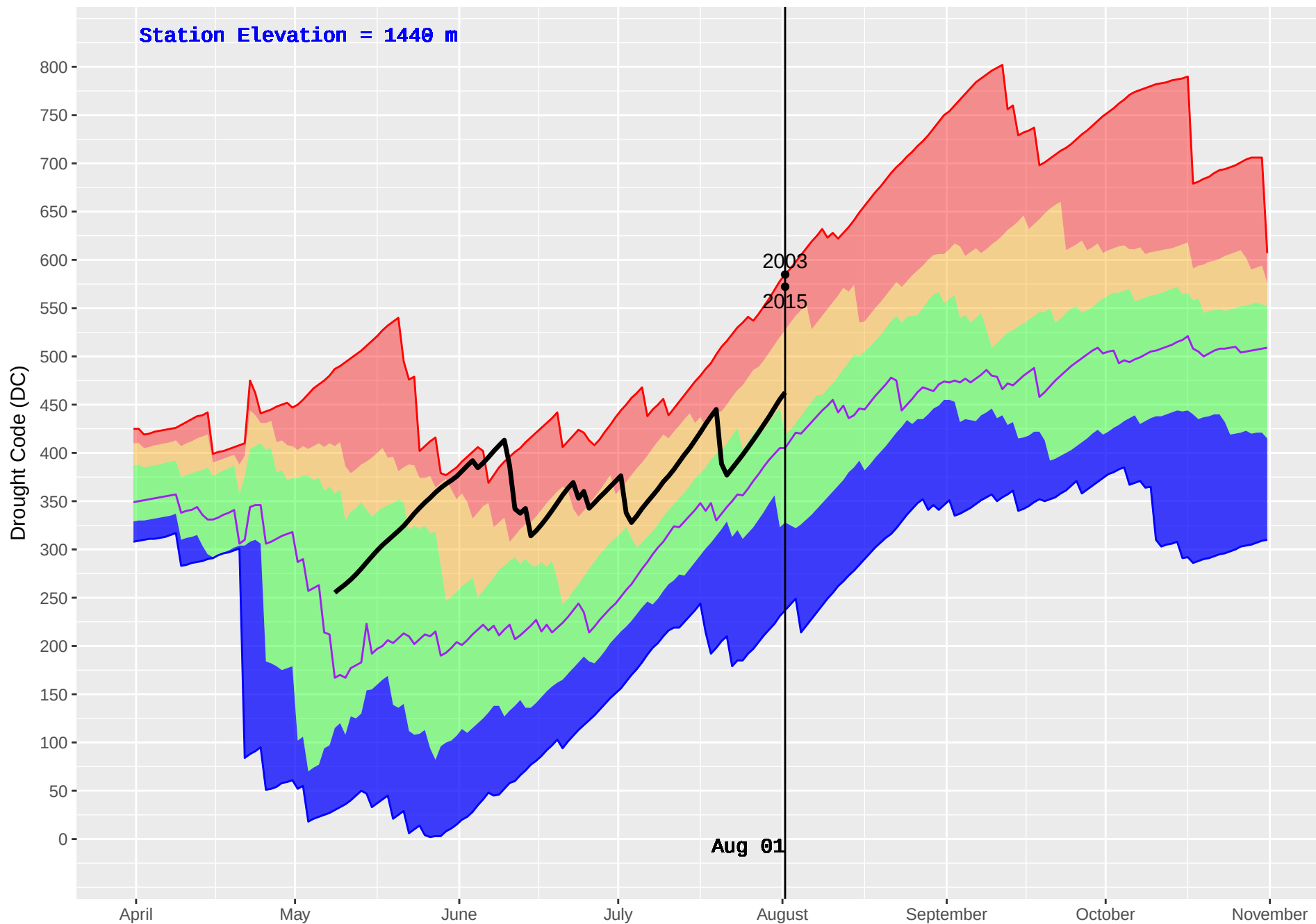
PASKA LAKE (326) : Historical (1999–2016) and Current (2018) Daily Drought Code (DC)
